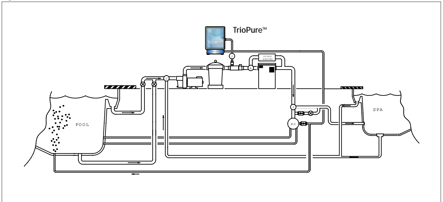
Figure 9 - (Existing Pool, Pool Spa Combination, ICS, Solar):
