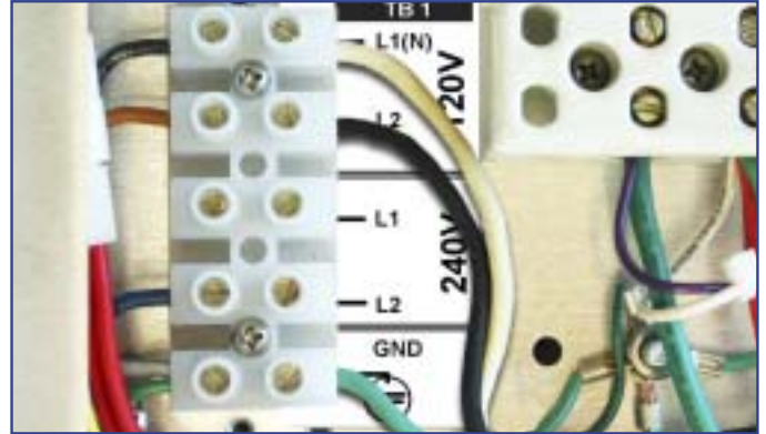
Figure - 11 Terminal Block 120V Configurations
