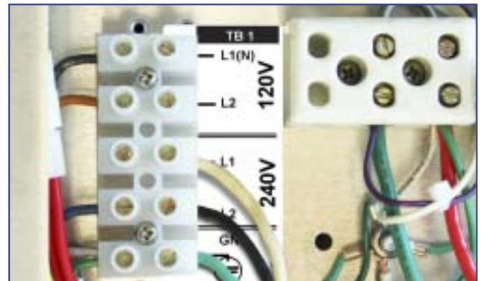
Figure - 12 Terminal Block 240V Configurations
