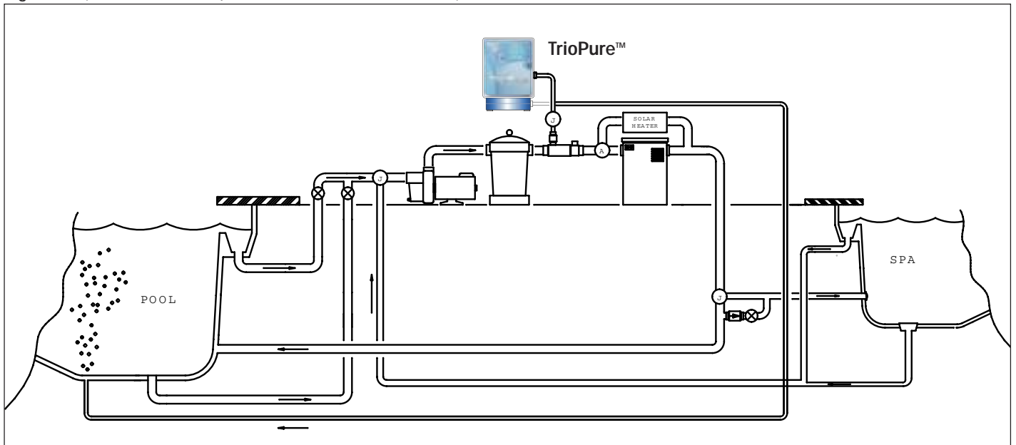
Figure 7 - (New Pool, Pool Spa Combination, No ICS, Solar):
