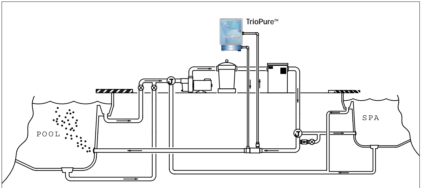
Figure 5 - (Existing Pool, Pool Spa Combination, No ICS, No solar):
