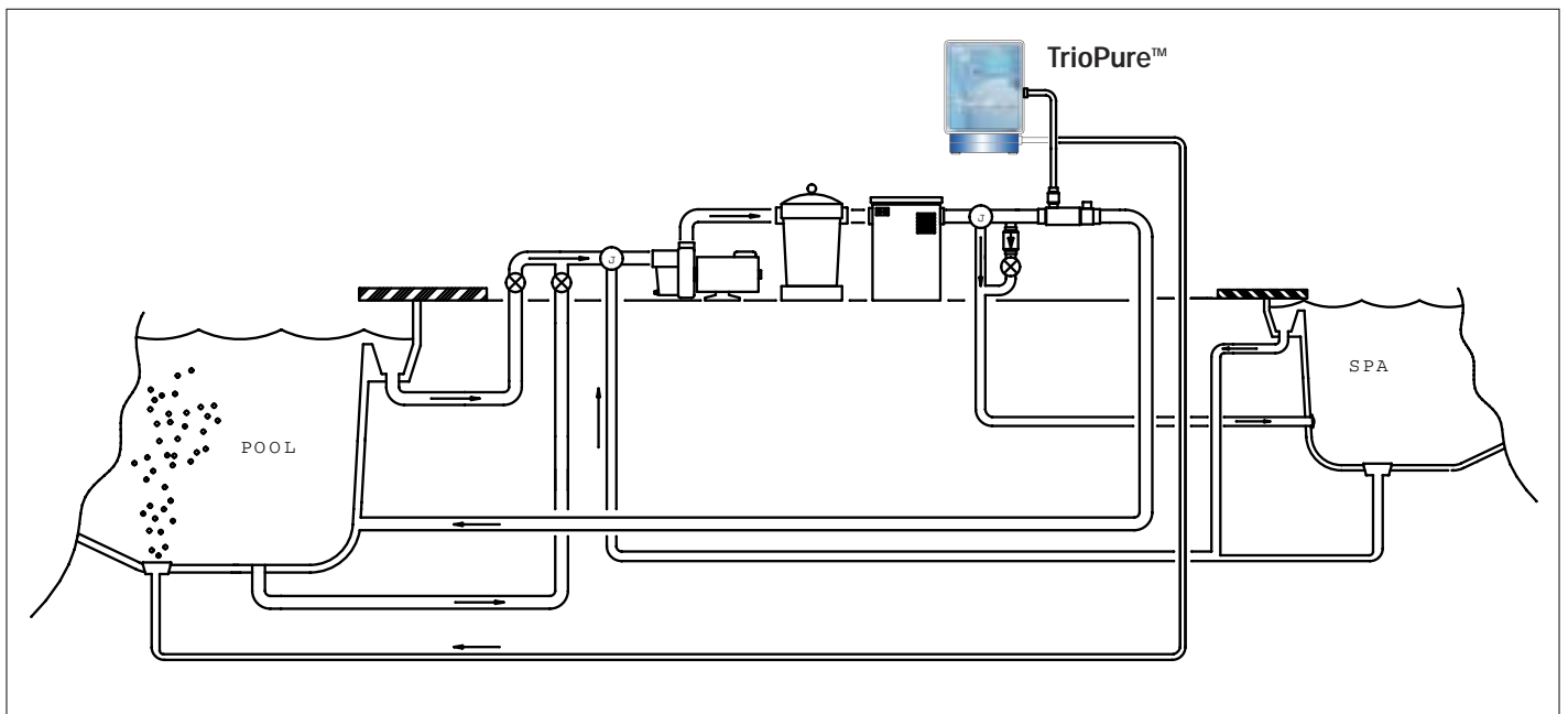
Figure 4 Description (New Pool, Pool Spa Combination, No ICS, No solar):
