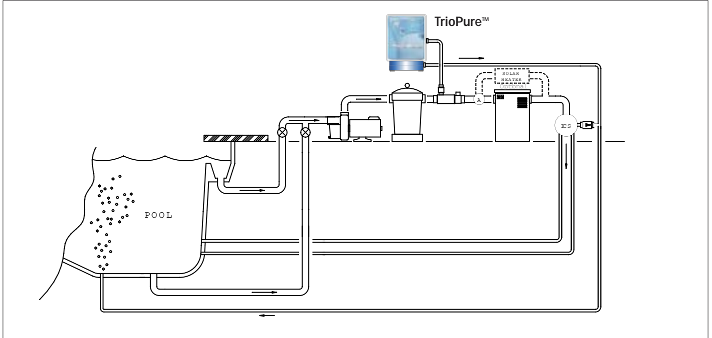
Figure 3 - (Existing Pool, Pool Only, ICS, Solar, No solar):
