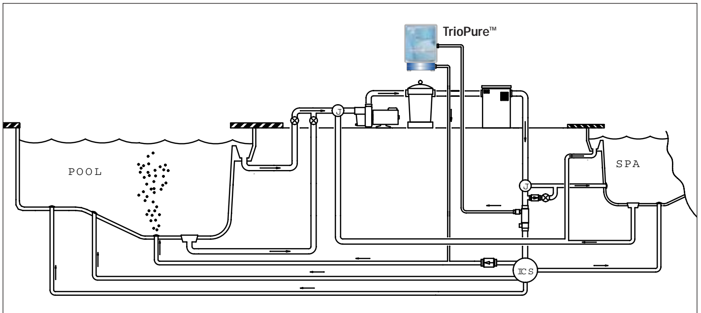
Figure 6 - (Existing Pool, Pool Spa Combination, ICS, No solar):
